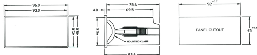
MECHANICAL SPECIFICATIONS
